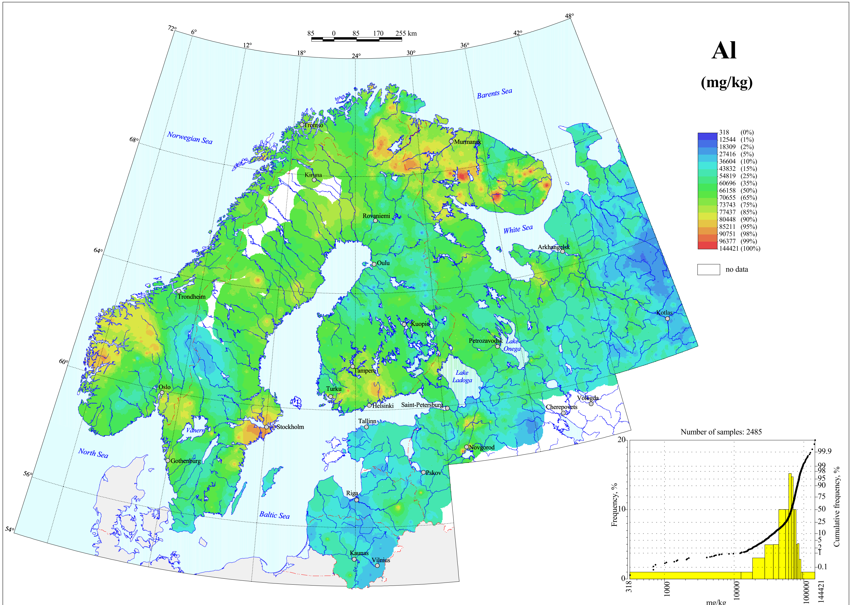
Aluminium in C-horizon, Grain Size <2 mm, Total Content
